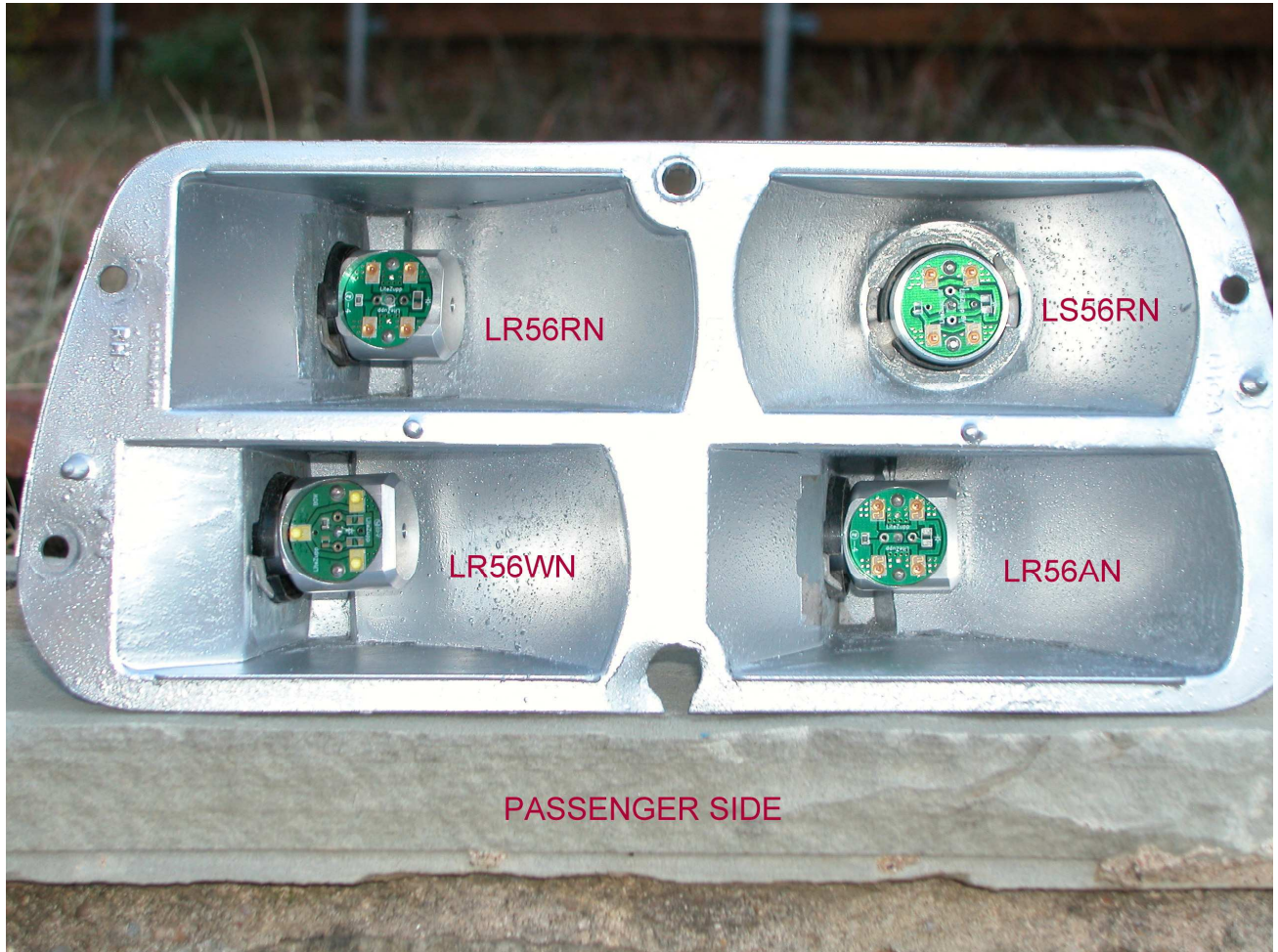
Passenger side layout of LED placement for the TR7
